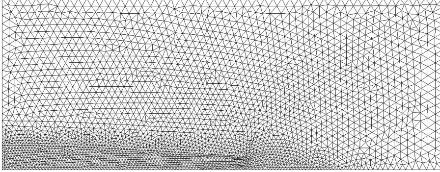
Figure 2: The computational mesh consisting of 6159 linear triangles at the computed pull-in position.
