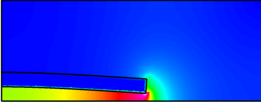
Figure 3: The magnitude of the electric field at the computed pull-in position.
