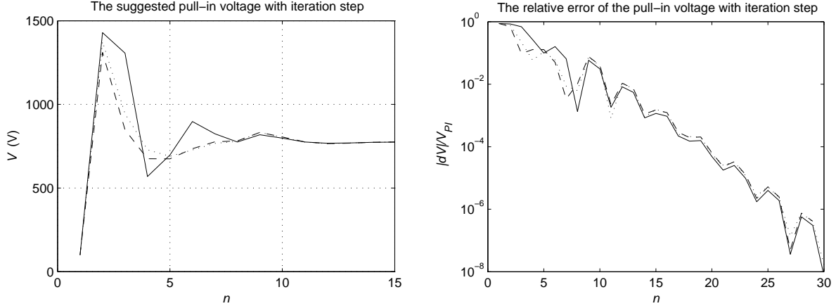
Figure 4: The convergence of the pull-in voltage with iteration step. The different lines represent cases with different number of sub-iterations for the pull-in position: solid line 1, dashed line 2 and dotted line 3.
