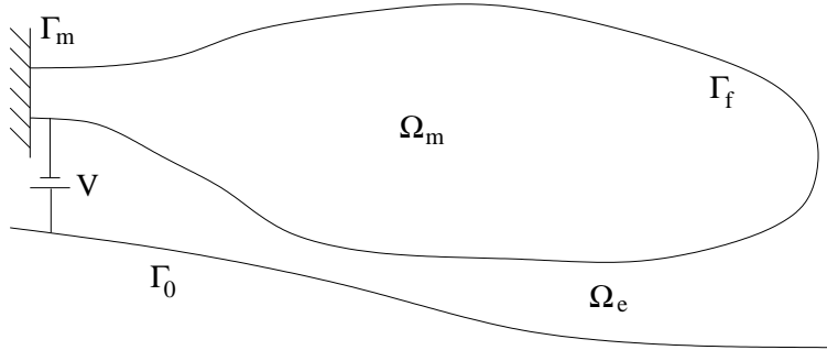
Figure 1: A schematic picture of the electro-mechanical system.
